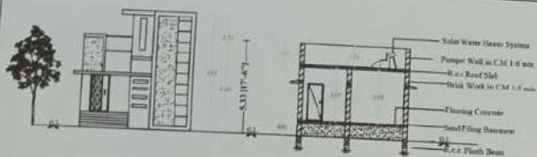
FRONT ELEVATION
