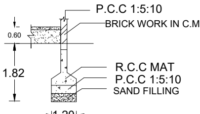
FOUNDATION DETAILS
