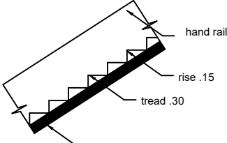
STAIR
