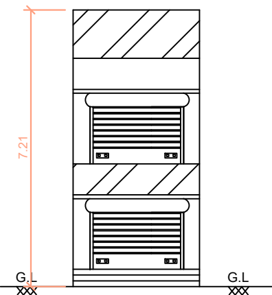
FRONT ELEVATION
