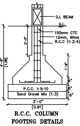
R.C.C. COLUMN FOOTING DETAILS SCALE : 1:25
