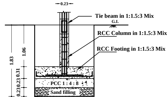
CROSS SECTION ON 'C-C'
