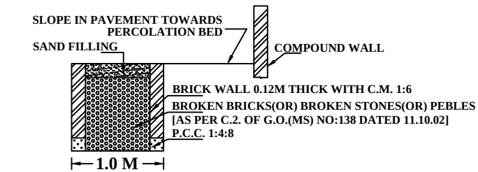
SECTION OF RAIN WATER PERCOLATION BED
