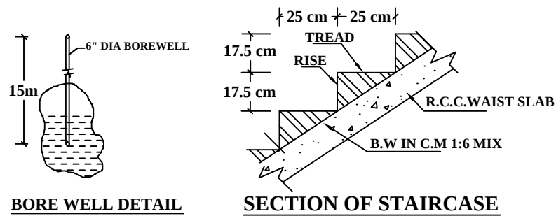
BORE WELL DETAIL
