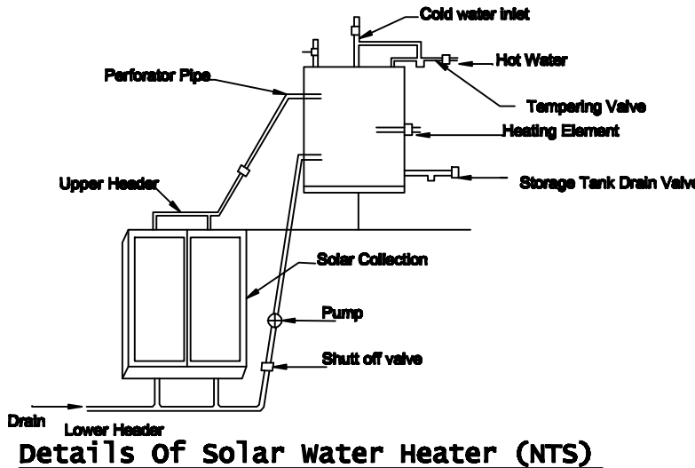
Details of solar water heater (NTS)
