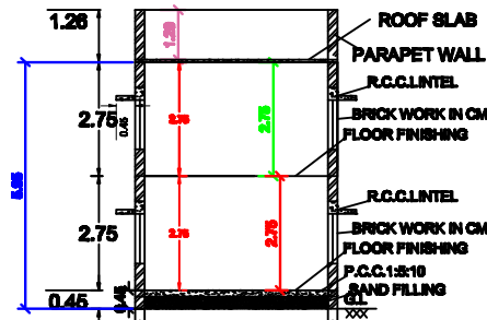
SECTION ON SS
