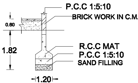
FOUNDATION DETAILS
