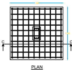
COLOUMN FOUNDATION DETAILS
