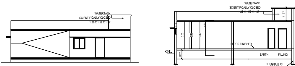
SECTION "AA"
