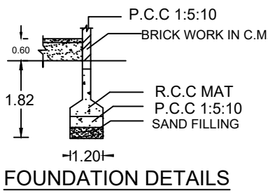
FOUNDATION DETAILS
