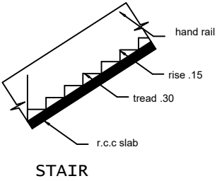
STAIR
