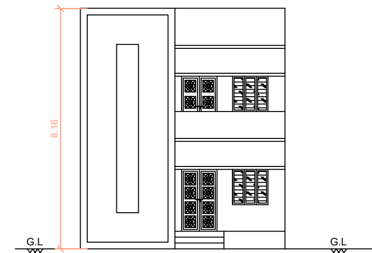
FRONT ELEVATION
