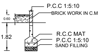
FOUNDATION DETAILS
