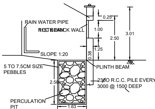
RAINWATER HARVESTING
