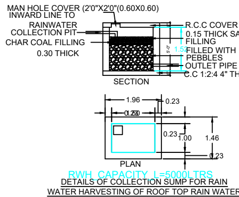
RAINWATER HARVESTING
