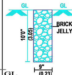
PERCULATION PIT
