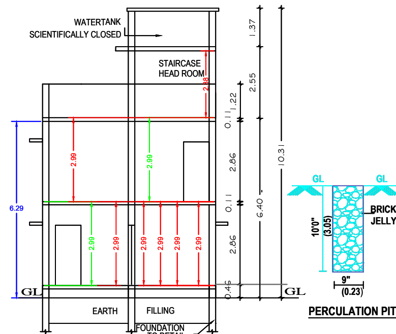
SECTION "A-B"
