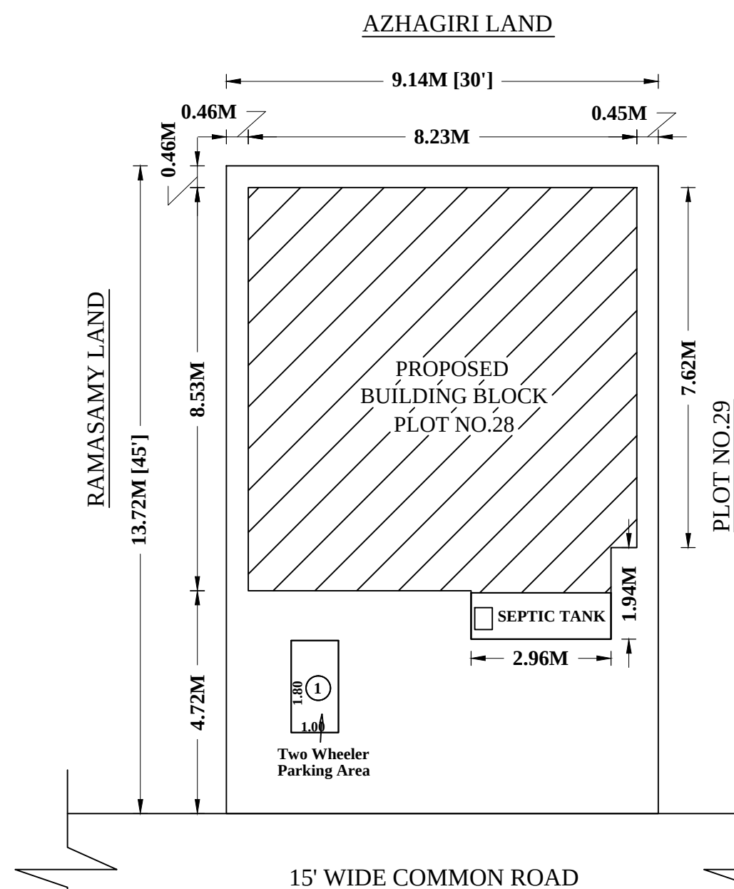
SITE PLAN SCALE IN -1:100
