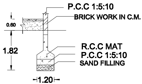
FOUNDATION DETAILS
