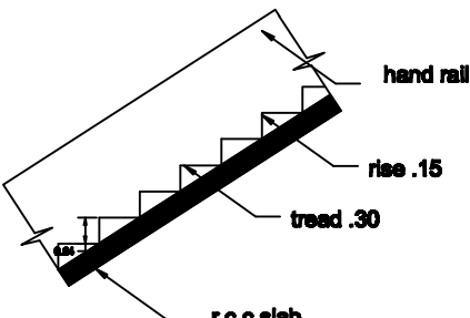
STAIR
