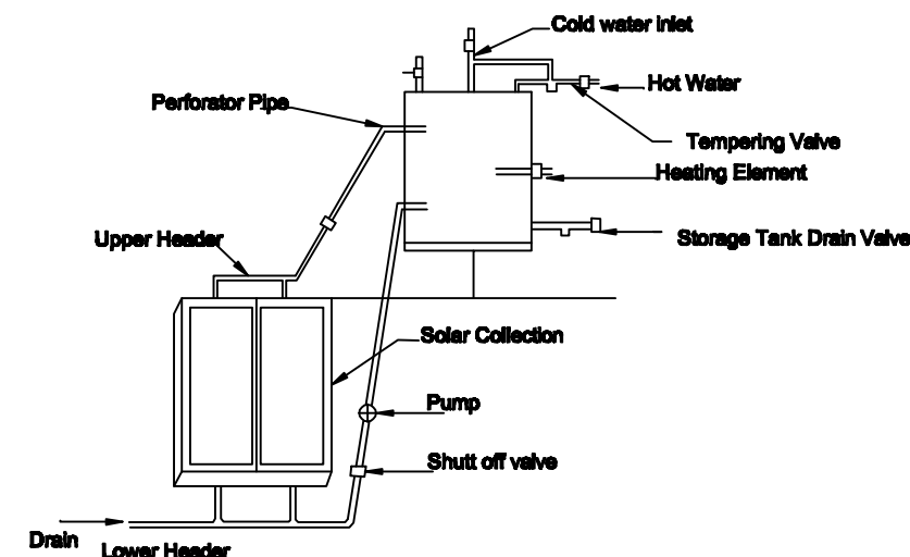
Details Of Solar Water Heater (NTS)
