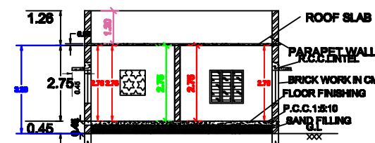
SECTION ON SS
