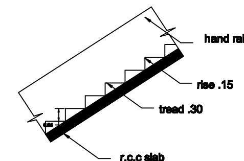
STAIR
