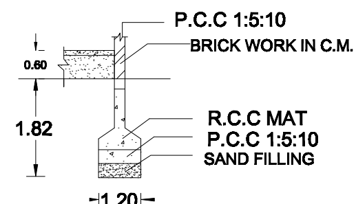
FOUNDATION DETAILS
