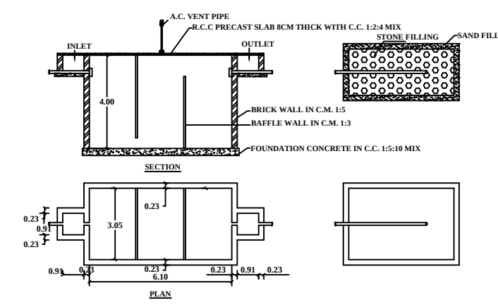
PLAN & SECTION OF SEPTIC TANK & DISPERSION TRENCH
