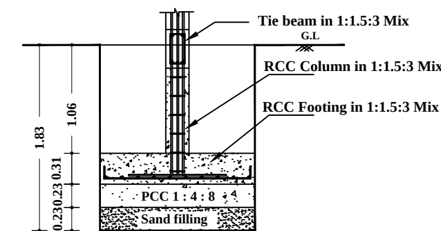
CROSS SECTION ON 'C - C'
