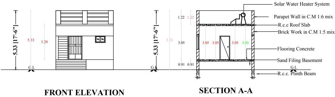
FRONT ELEVATION
