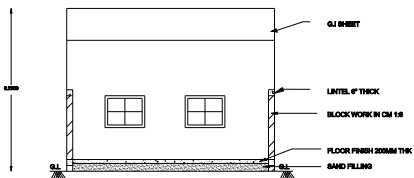
CROSS SECTION - AB
