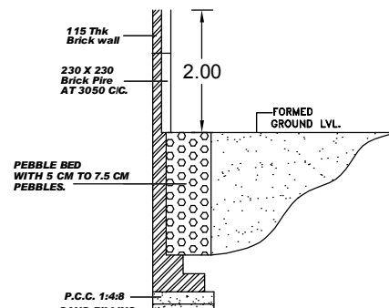
SECTION OF COMPOUND WALL & RAINWATER COLLECTING PIT
