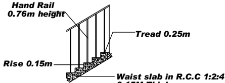
STAIRCASE SECTION
