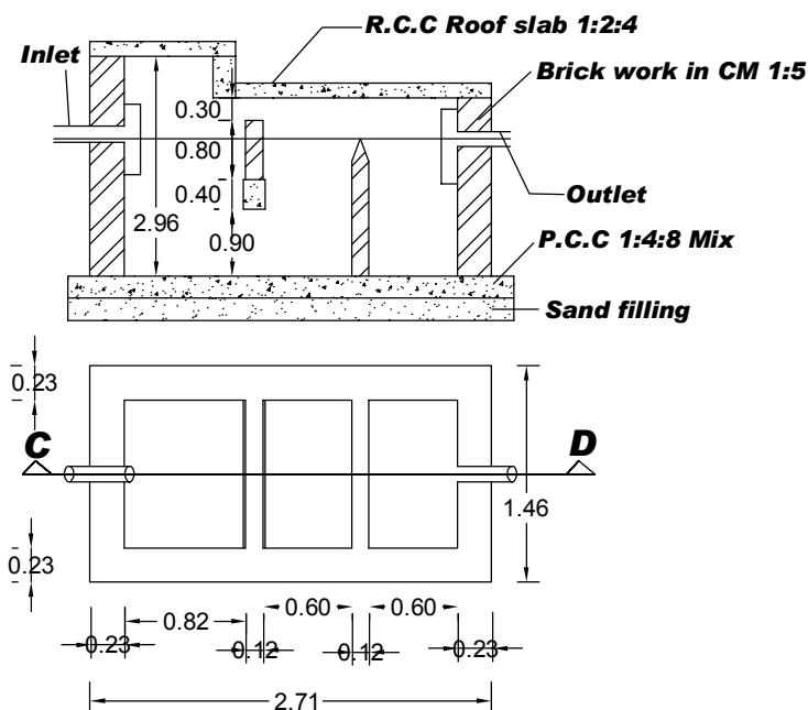
SEPTIC TANK DETAILS [SCALE 1:50]
