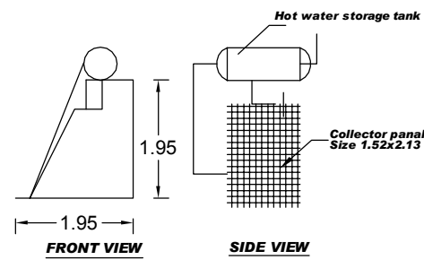
SOLAR WATER HEATER DETAILS [SCALE 1:100]
