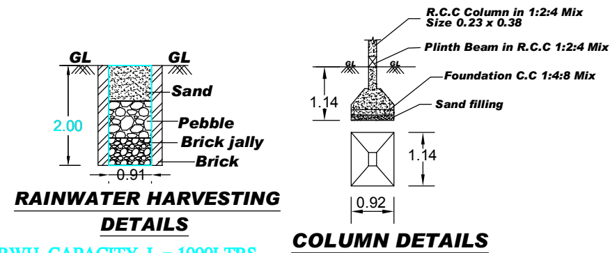
COLUMN DETAILS
