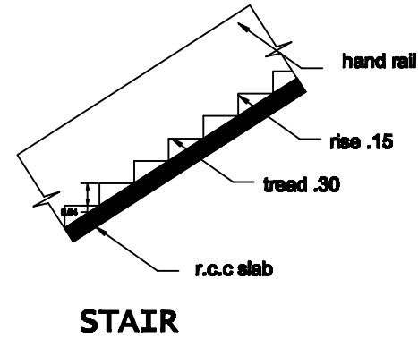
STAIR
