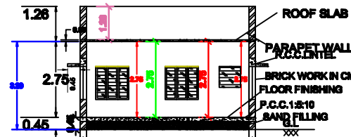
SECTION ON SS
