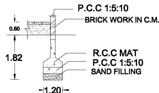
FOUNDATION DETAILS
