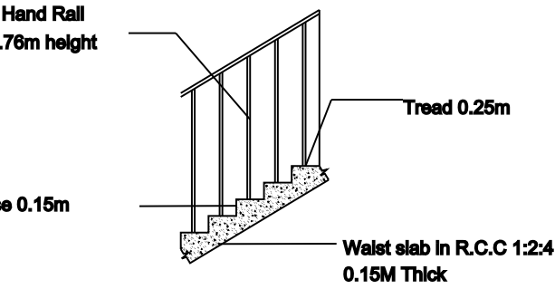
STAIRCASE SECTION
