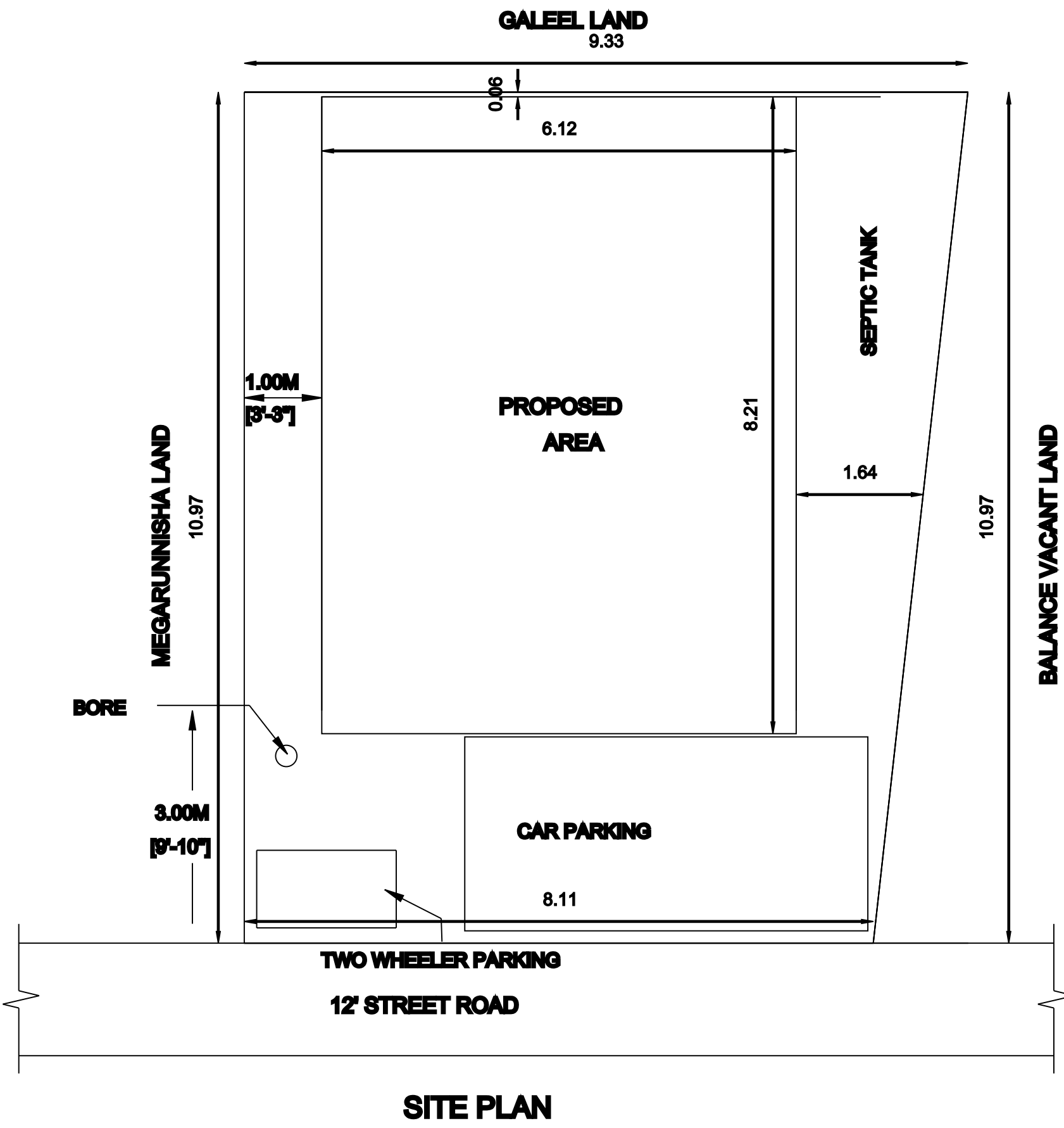
SITE PLAN
