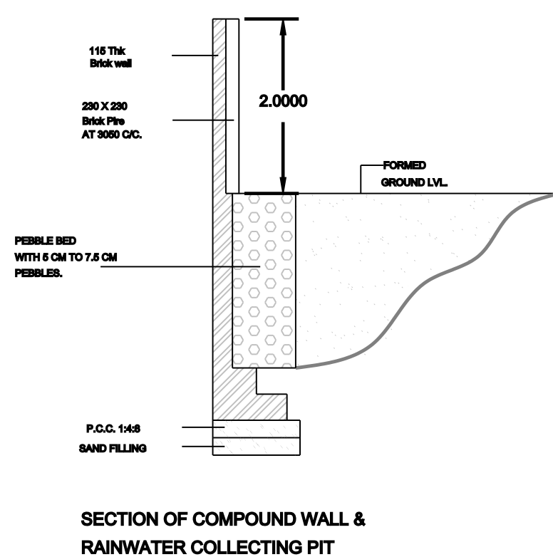
SECTION OF COMPOUND WALL & RAINWATER COLLECTING PIT
