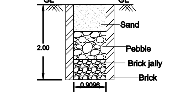
RAINWATER HARVESTING DETAILS
