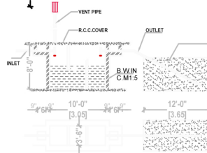
SEPTIC TANK & D-TRENCH DETAILS (NOT TO SCALE)
