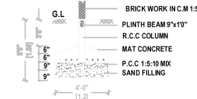
COLUMN FOUNDATION (NOT TO SCALE)
