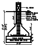
R.C.C. COLUMN DETAIL
