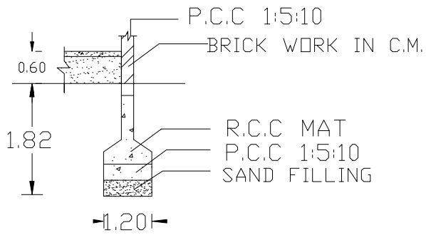
FOUNDATION DETAILS
