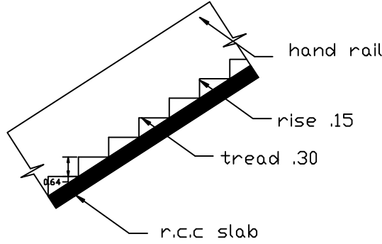
STAIR
