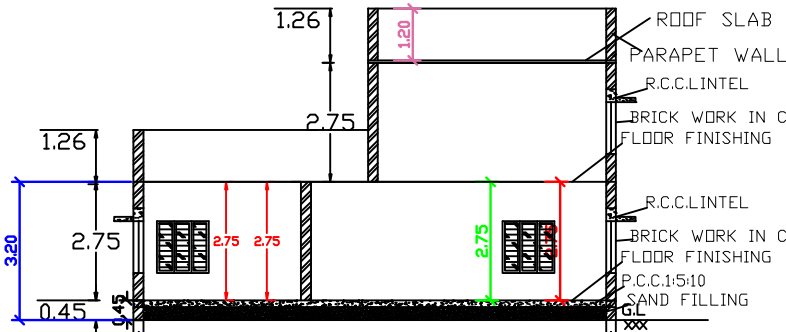
SECTION ON SS
