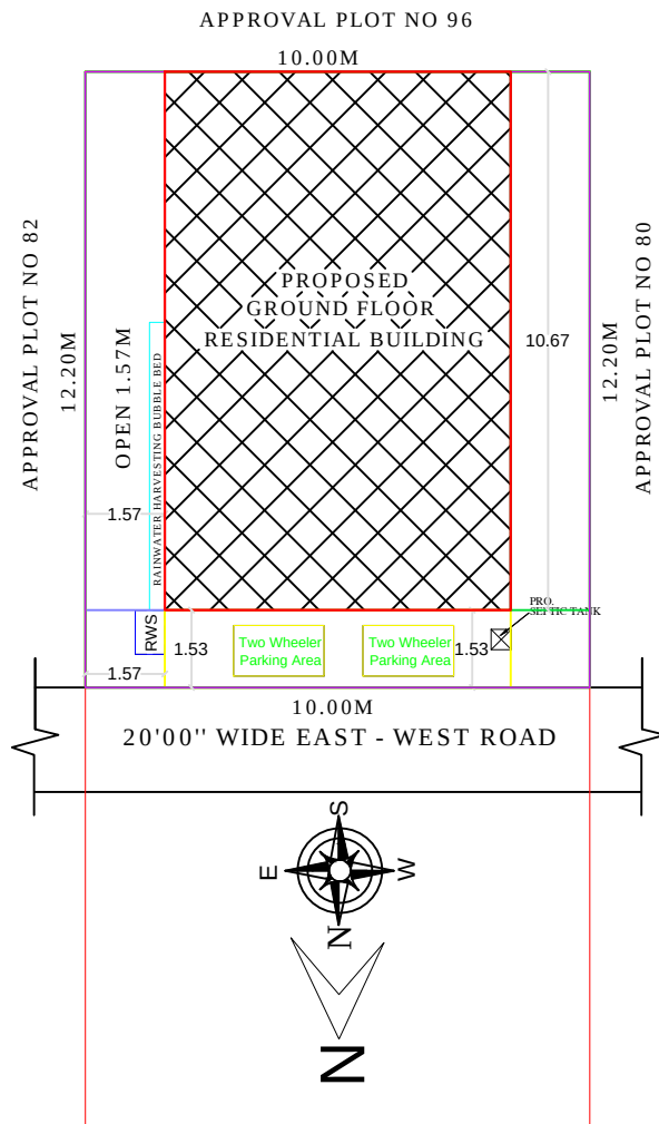
SITE PLAN
