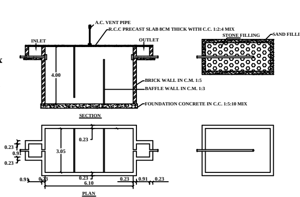
PLAN PLAN & SECTION OF SEPTIC TANK & DISPERSION TRENCH
