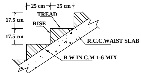
SECTION OF STAIRCASE
