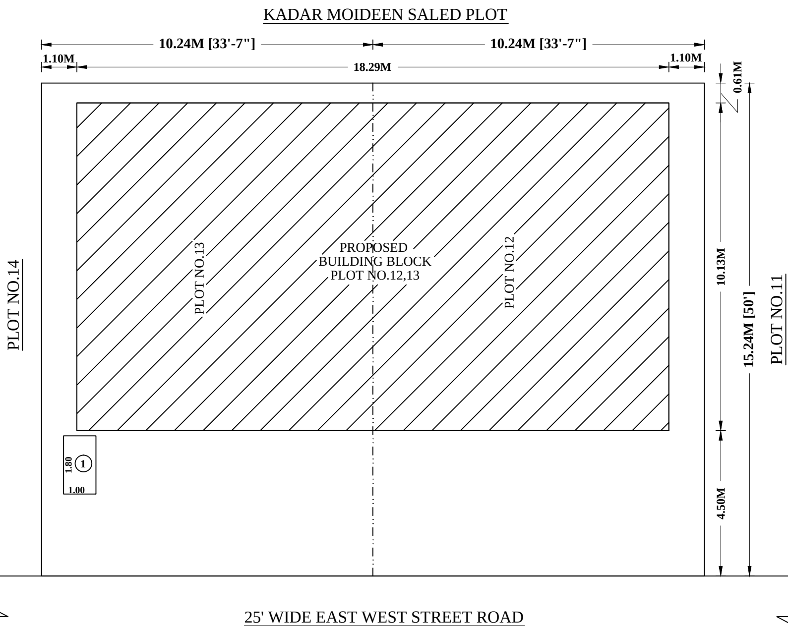
SITE PLAN SCALE IN -1:100
