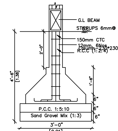
R.C.C. COLUMN FOOTING DETAILS SCALE : 1:25
