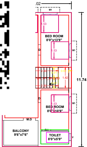
PRO. FIRST FLOOR PLAN.
