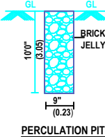
PERCOLATION PIT
