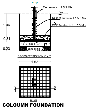
COLOUMN FOUNDATION
