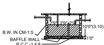
SEPTIC TANK SECTION-(XY)
