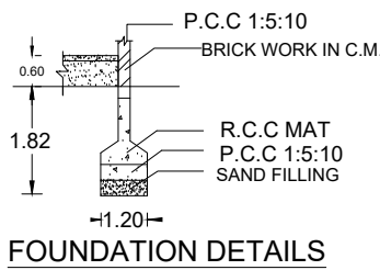
FOUNDATION DETAILS
