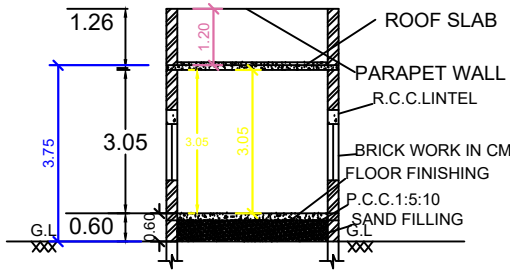
SECTION ON SS
