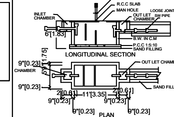
SEPTIC TANK:
