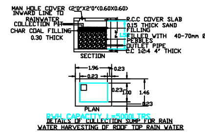
DETAILS OF COLLECTION SUM FOR RAIN WATER HARVESTING OF ROOF TOP RAIN WATER
