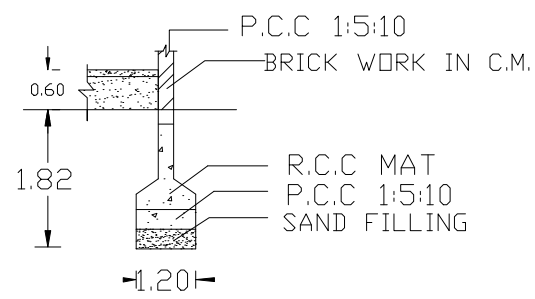
FOUNDATION DETAILS
