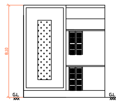
FRONT ELEVATION
