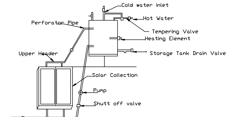
Details Of Solar Water Heater (NTS)
