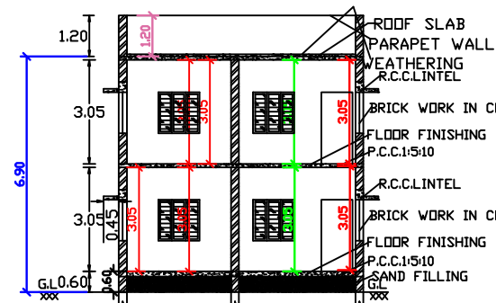
SECTION ON SS
