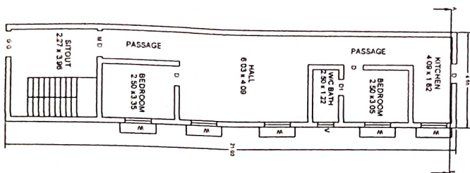
PRO. GROUND FLOOR PLAN
