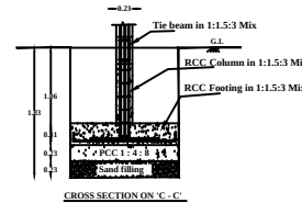
COLOUMN FOUNDATION DETAILS
