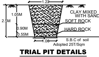
TRIAL PIT DETAILS
