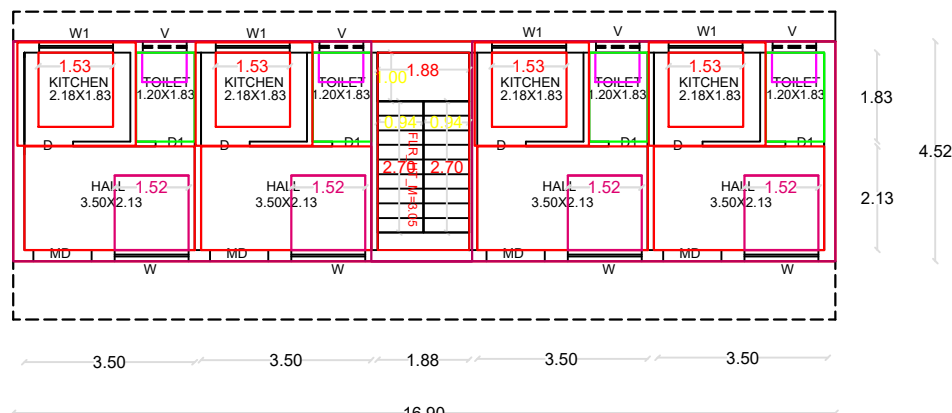
PRO-FIRST FLOOR PLAN
