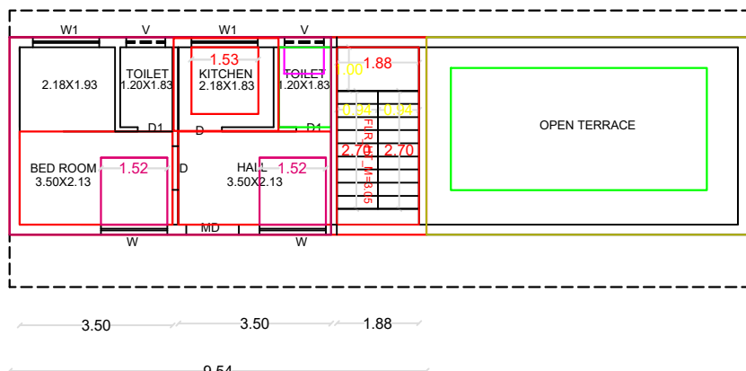
SECOND CUM TERRACE FLOOR PLAN
