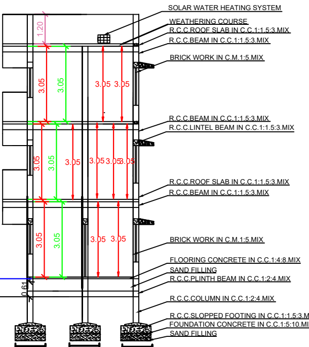
SRCTION ON 'AA'
