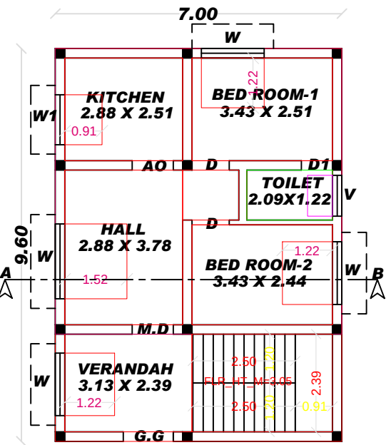
PRO.GROUND FLOOR PLAN (NORTH FACING)
