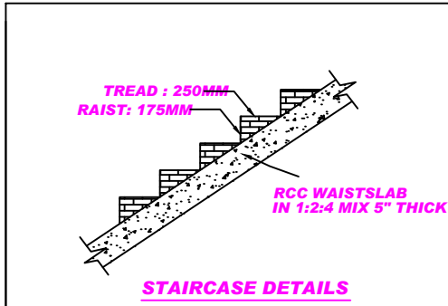
STAIRCASE DETAILS
