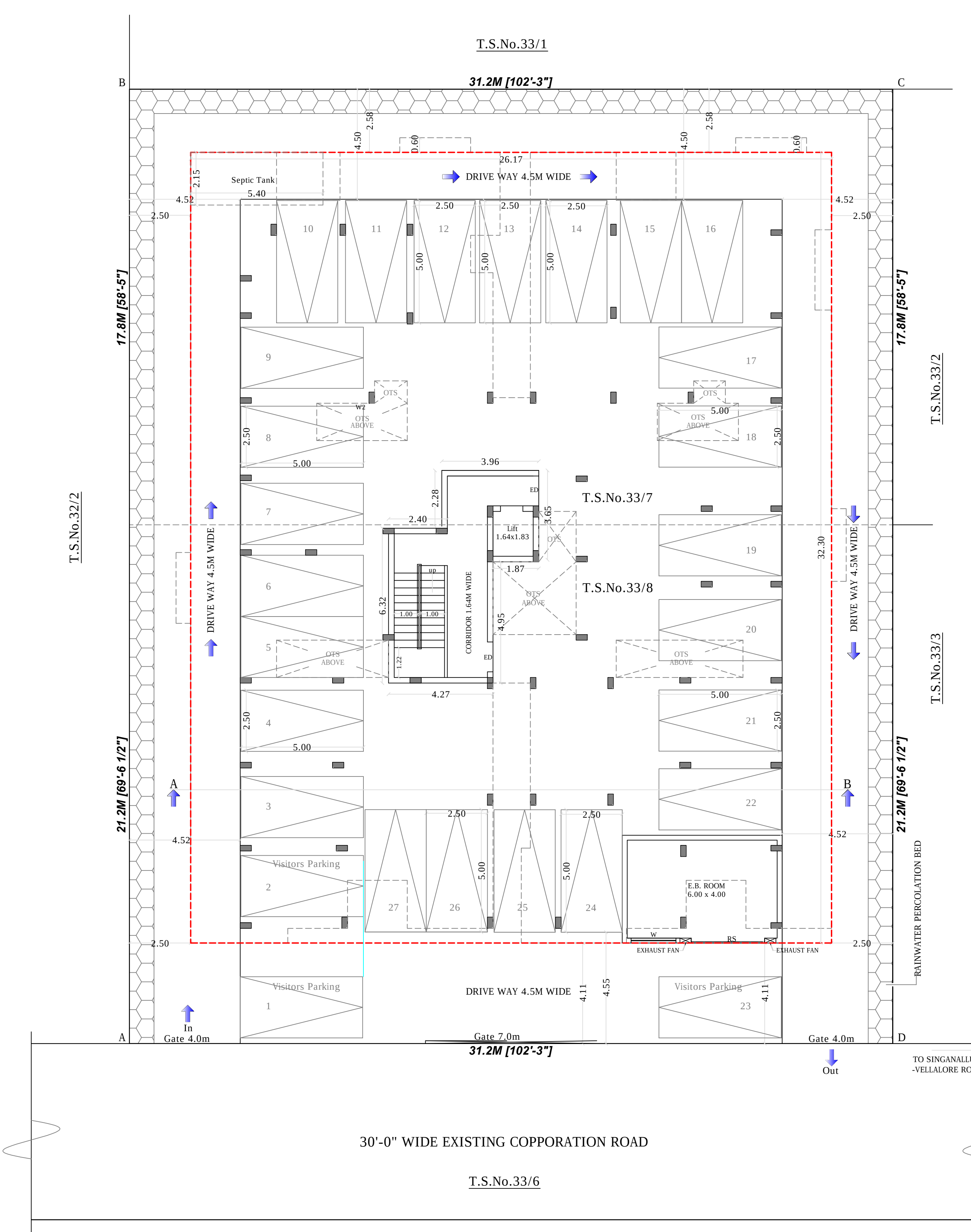
SITE/STILT FLOOR PLAN
