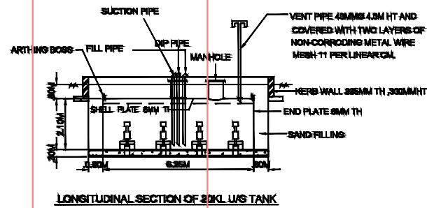
LONGITUDINAL SECTION OF BORE WELL TANK
