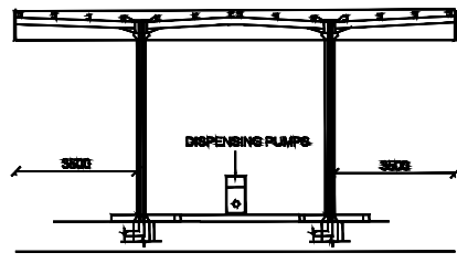
SECTION 'XX' CANOPY DETAIL (NOT TO SCALE)
