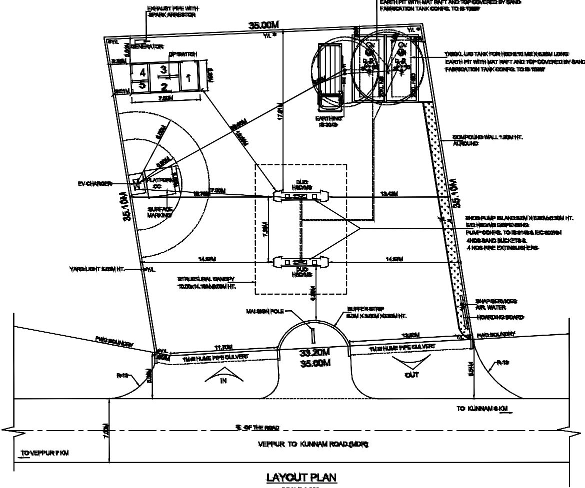
LAYOUT PLAN SCALE 1:500
