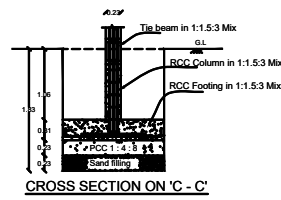
CROSS SECTION ON 'C-C'
