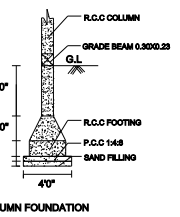
COLOUMN FOUNDATION DETAILS
