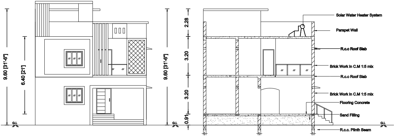
FRONT ELEVATION
