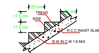
SECTION OF STAIRCASE
