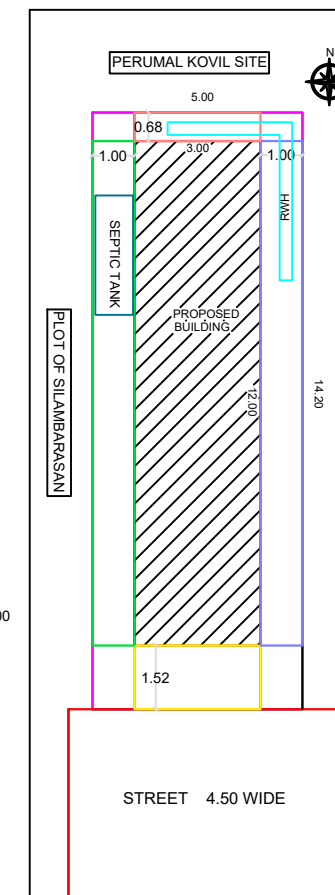
SITE PLAN
