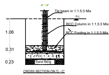
CROSS SECTION ON 'C-C'
