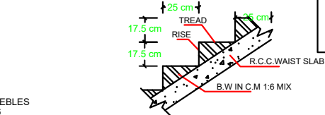
SECTION OF STAIRCASE
