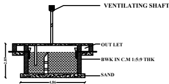
SECTION OF THE SEPTIC TANK
