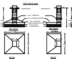
COLUMN FOOTING DETAILS
