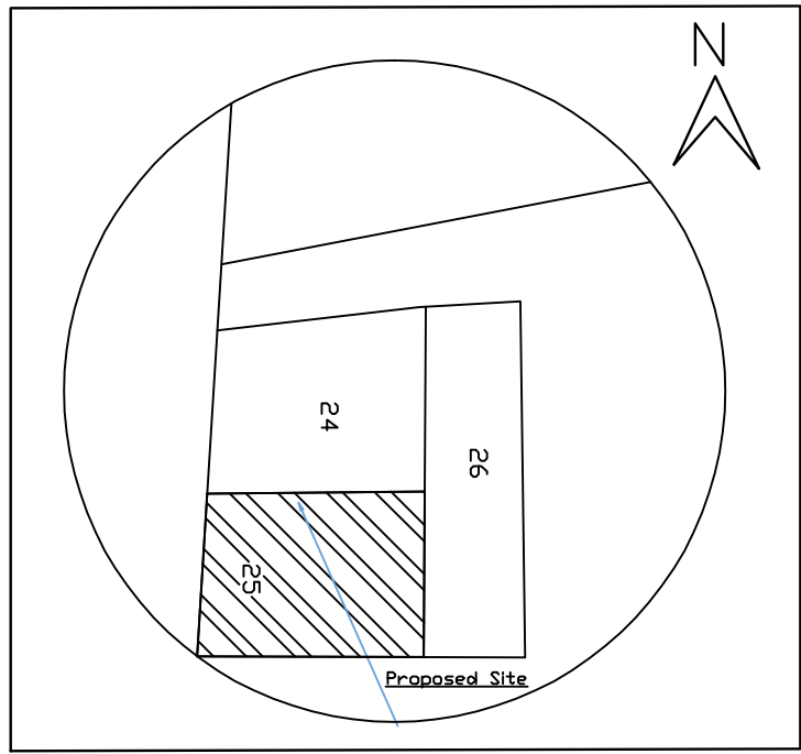
TOPO PLAN:
