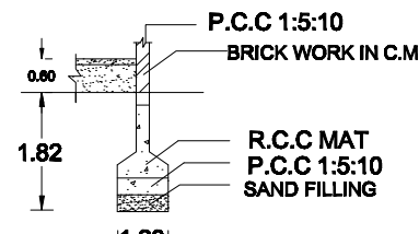
FOUNDATION DETAILS
