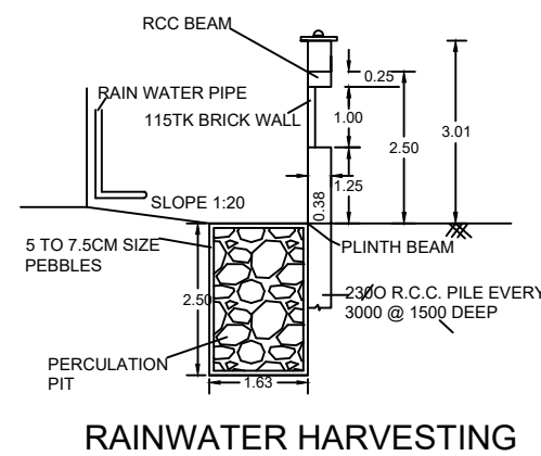
RAINWATER HARVESTING
