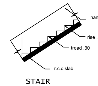
STAIR
