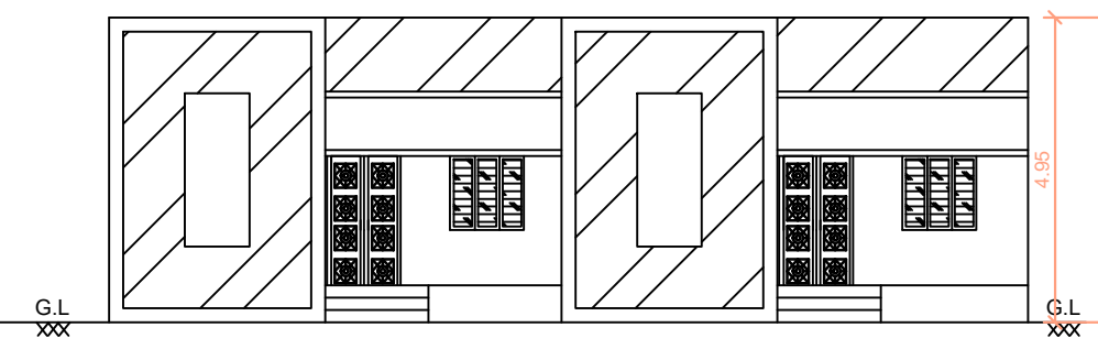
FRONT ELEVATION
