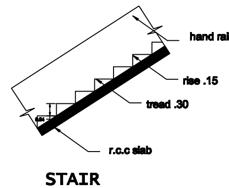
STAIR
