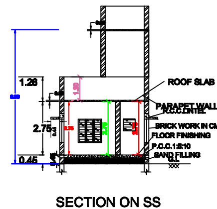
SECTION ON SS
