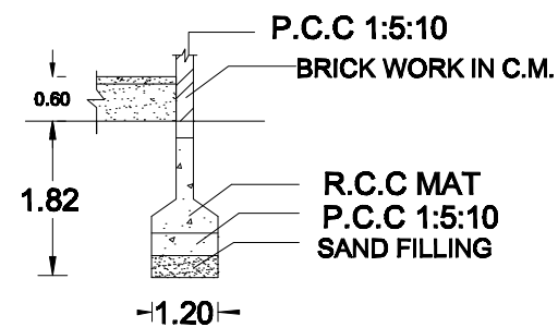
FOUNDATION DETAILS
