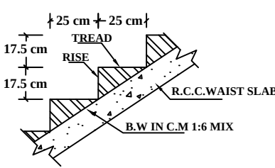
SECTION OF STAIRCASE
