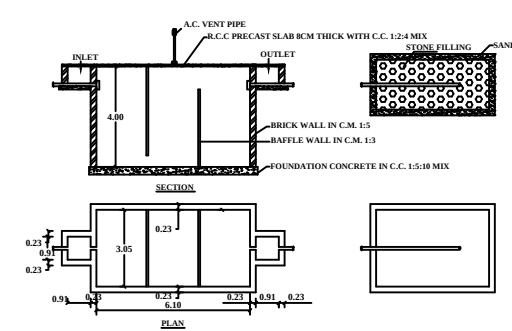
PLAN & SECTION OF SEPTIC TANK & DISPERSION TRENCH
