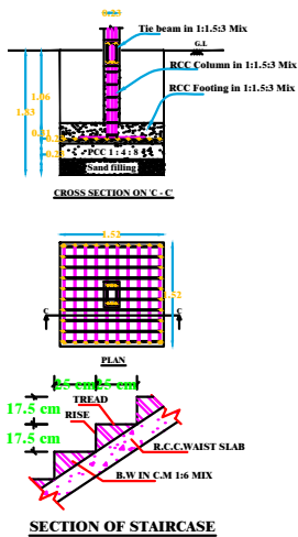
SECTION OF STAIRCASE
