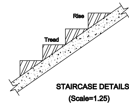
STAIRCASE DETAILS (Scale=1:25)
