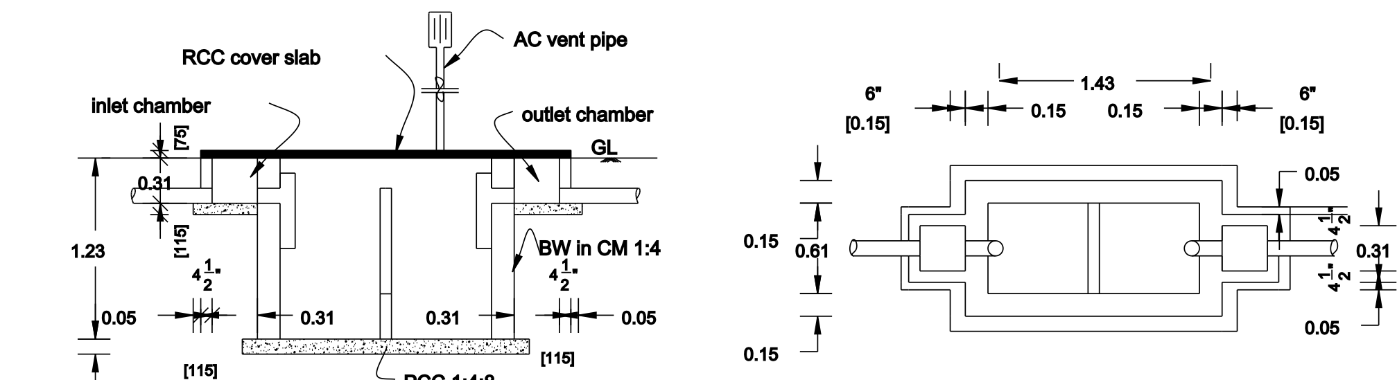
SEPTIC TANK DETAILS
