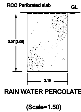
RAIN WATER PERCOLATED PIT (Scale=1:50)
