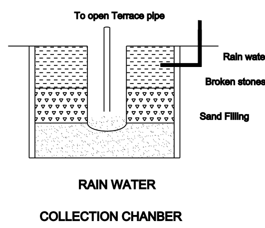
RAIN WATER COLLECTION CHAMBER
