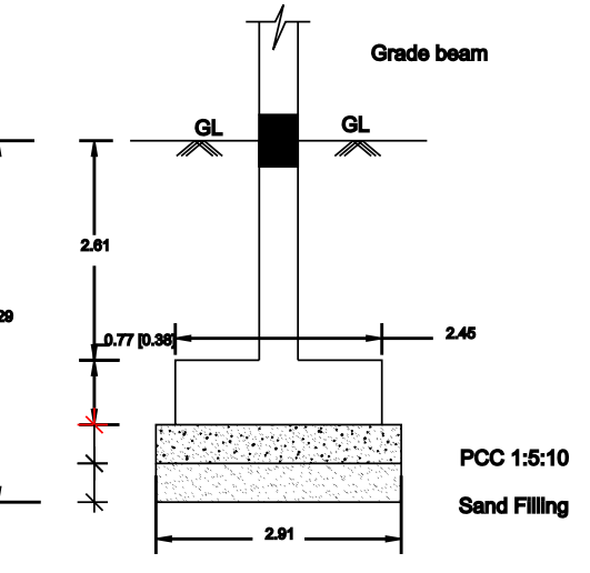
FOUNDATION DETAILS (Scale=1:50)
