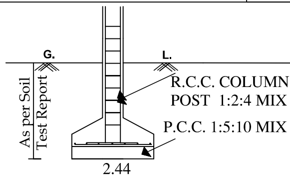
COLUMN POST DETAILS
