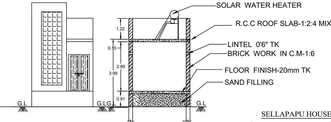
CROSS SECTION (A-B)
