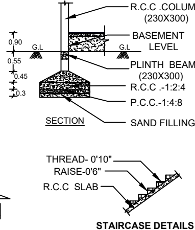
STAIRCASE DETAILS
